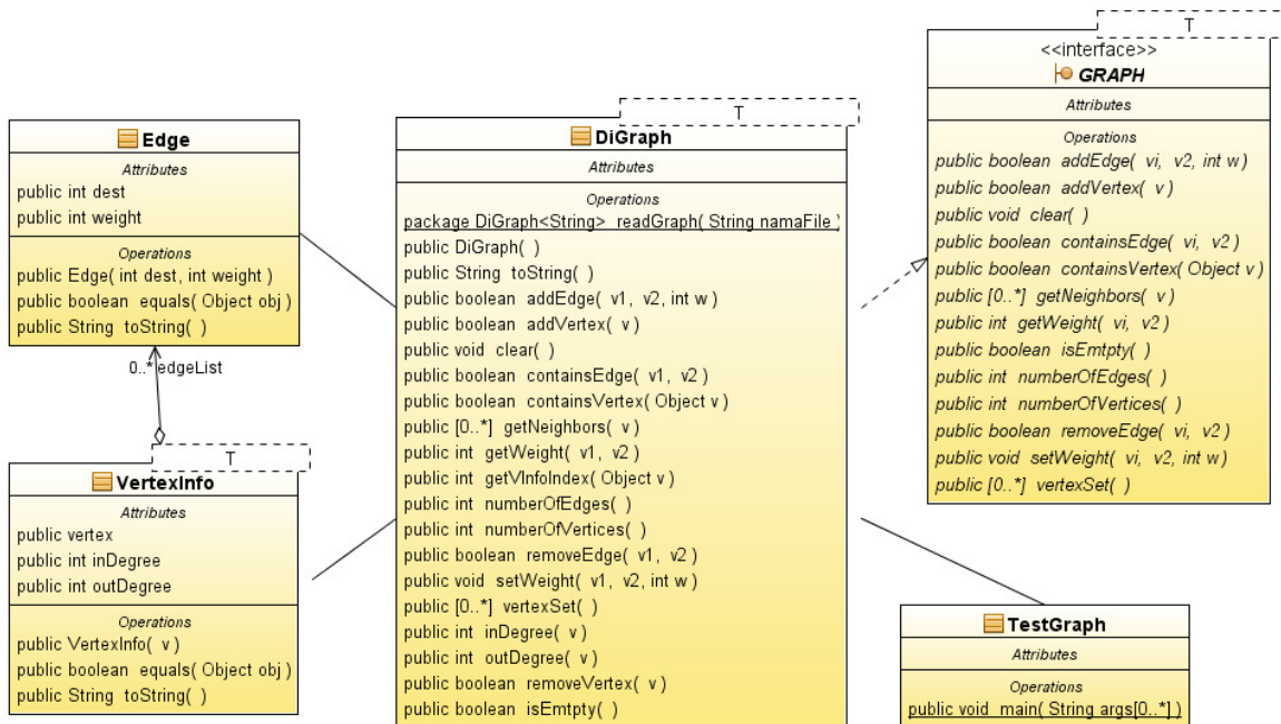
Gambar 29.15 Diagram UML Implementasi Graph
