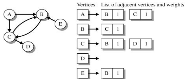
Gambar 29.11 Graph 1 dan List Adjacency
