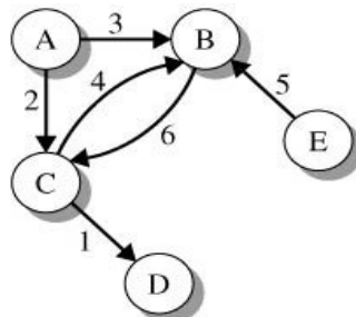
Gambar 29.16 Contoh Graph
