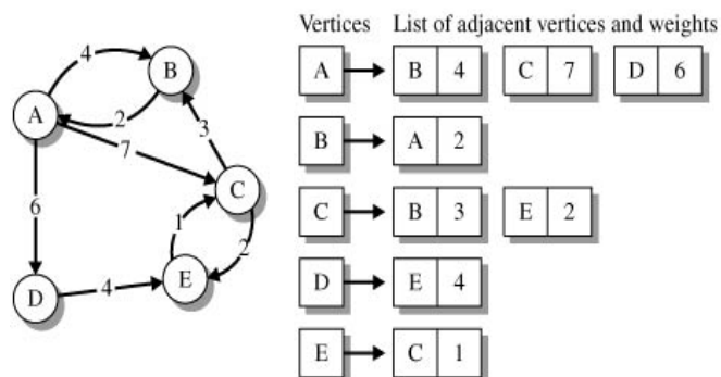
Gambar 29.12 Graph 2 dan List Adjacency
