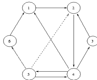
Gambar 29.5 Graph berarah
