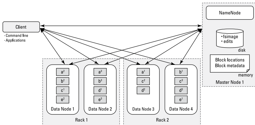
Figure 4-4: Interaction between HDFS components.
