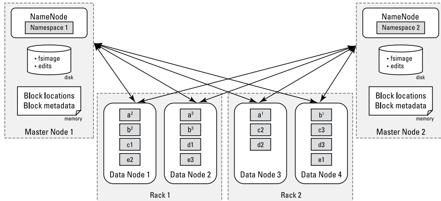
Figure 4-6: Replication patterns of data blocks in HDFS.
