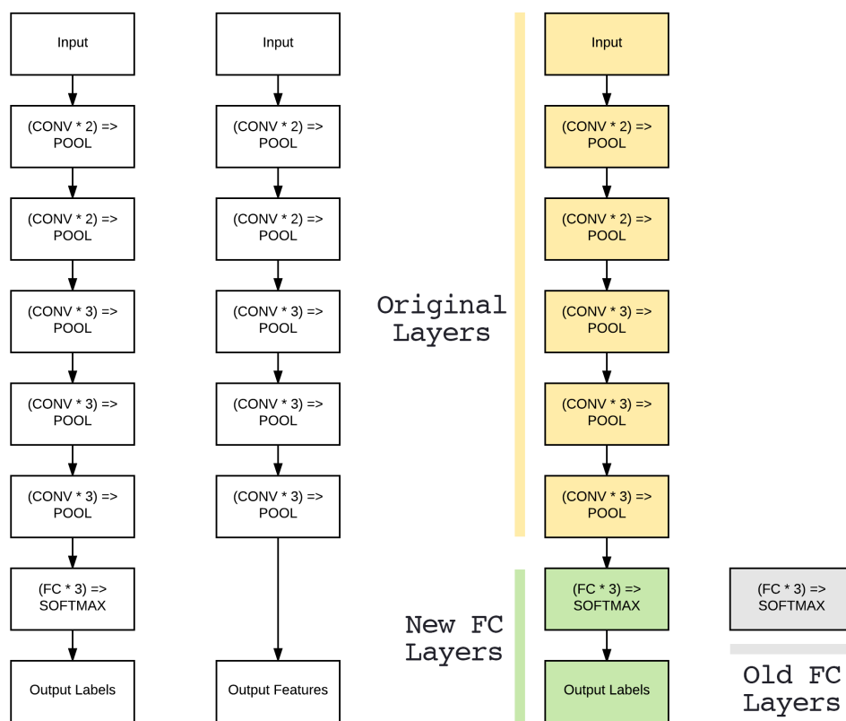
Figure 5.1: Left: The original VGG16 network architecture. Middle: Removing the FC layers from VGG16 and treating the final POOL layer as a feature extractor. Right: Removing the original FC layers and replacing them with a brand new FC head. These new FC layers can then be fine-tuned to the specific dataset (the old FC layers are no longer used).
