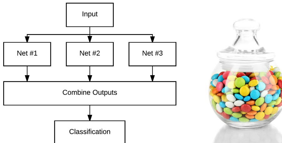
Figure 6.2: Left: An ensemble of neural networks consists of multiple networks. When classifying an input image the data point is passed to each network where it classifies the image independently of all other networks. The classifications across networks are then averaged to obtain the final prediction. Right: Ensemble methods are possible due to Jensen’s Inequality. By averaging guesses as to the number of candies in the jar, we can better approximate the true number of candies.
