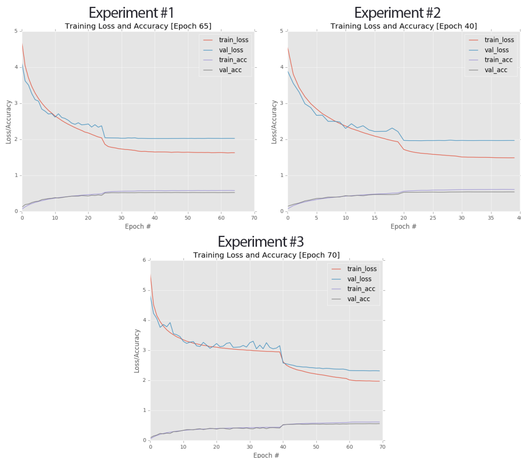
Figure 11.12: Top-left: Plots for Experiment #1. Top-right: Learning curves for Experiment #2. Bottom: Training/validation plots for Experiment #3. The final experiment obtains the best validation accuracy at 55.77%.
