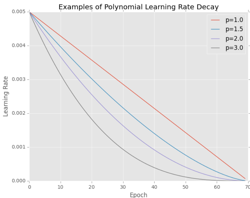
Figure 11.6: Plots of polynomial learning rate decays for varying values of the power, p . Notice how as the power increases the sharper the decay. Setting p = 1.0 turns a polynomial decay into a linear decay.
