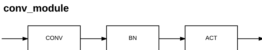
Figure 11.3: The conv_module of the MiniGoogLeNet architecture. This module includes no branching and is a simple CONV => BN => ACT .
