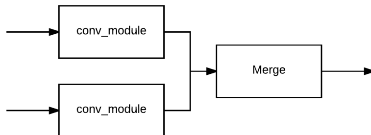
Figure 11.4: The (mini)-inception_module consists of two branches. The first branch is a CONV layer responsible for learning 1 \times 1 filters. The second branch is another CONV layer that learns 3 \times 3 filters. The filter responses are then concatenated along the channel dimension.
