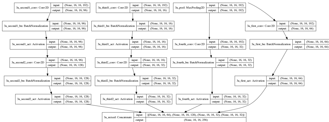
Figure 11.11: The full Inception module proposed by Szegedy et al. (zoomed out to save space). The key takeaway here is that there are four distinct branches in the Inception module.
