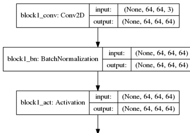
Figure 11.10: A sample of the DeeperGoogLeNet architecture visualization which includes the actual names for each layer. Naming layers makes it easier to keep track of them in larger, deeper networks.
