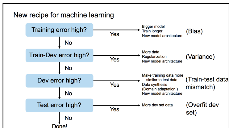
Figure 8.2: Slide 13 of Andrew Ng’s talk [34]. Here Ng proposes four separate data splits when training a deep learning model.
