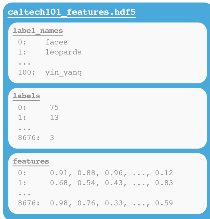
Figure 3.2: An example of a HDF5 file with three datasets. The first dataset contains the label_names for CALTECH-101. We then have labels , which maps the each image to its corresponding class label. Finally, the features dataset contains the image quantifications extracted by the CNN.
