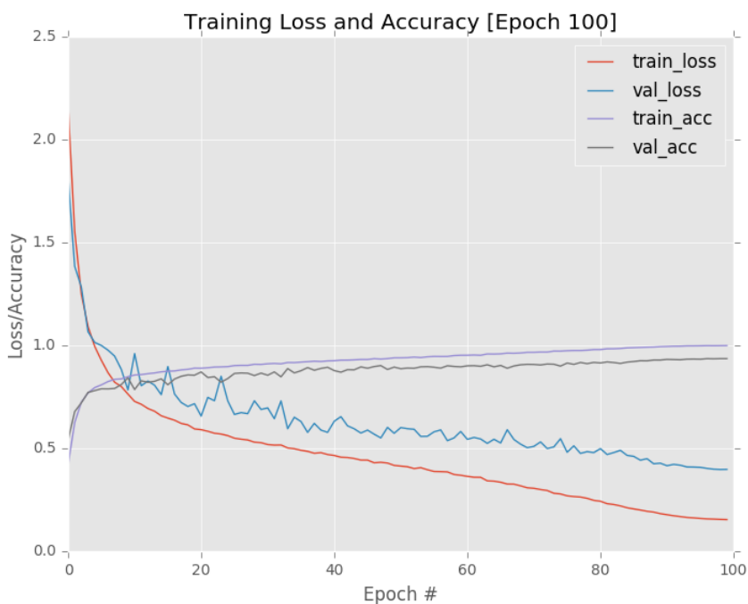
Figure 12.7: Training ResNet on CIFAR-10 using learning rate decay beats out all previous experiments.
