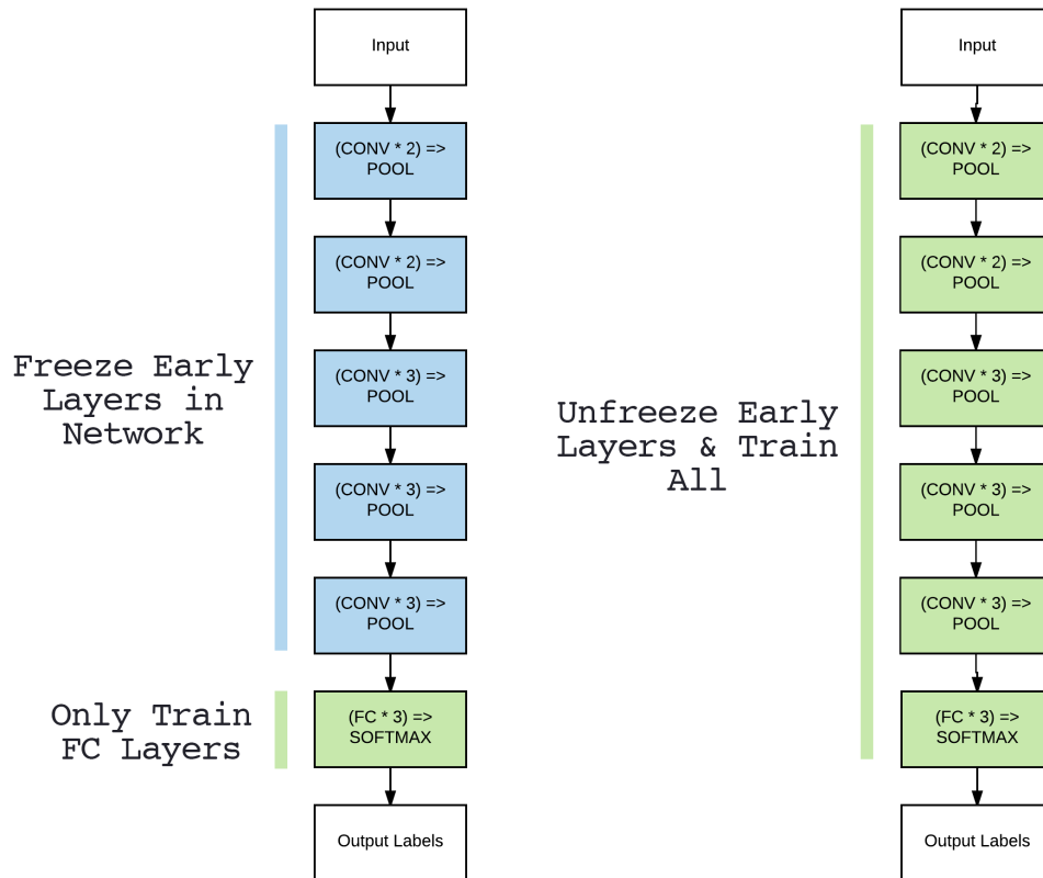
Figure 5.2: Left: When we start the fine-tuning process we freeze all CONV layers in the network and only allow the gradient to backpropagate through the FC layers. Doing this allows our network to “warm up”. Right: After the FC layers have had a chance to warm up we may choose to unfreeze all layers in the network and allow each of them to be fine-tuned as well.
