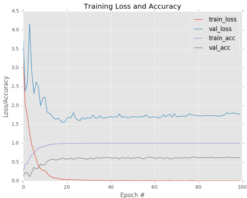
Figure 2.5: Learning plot for MiniVGGNet applied to the Flowers-17 dataset without data augmentation. Notice how overfitting starts to occur past epoch 25 as our validation loss increases.
