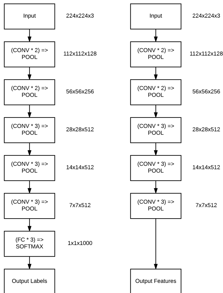
Figure 3.1: Left: The original VGG16 network architecture that outputs probabilities for each of the 1,000 ImageNet class labels. Right: Removing the FC layers from VGG16 and instead returning the output of the final POOL layer. This output will serve as our extracted features.
