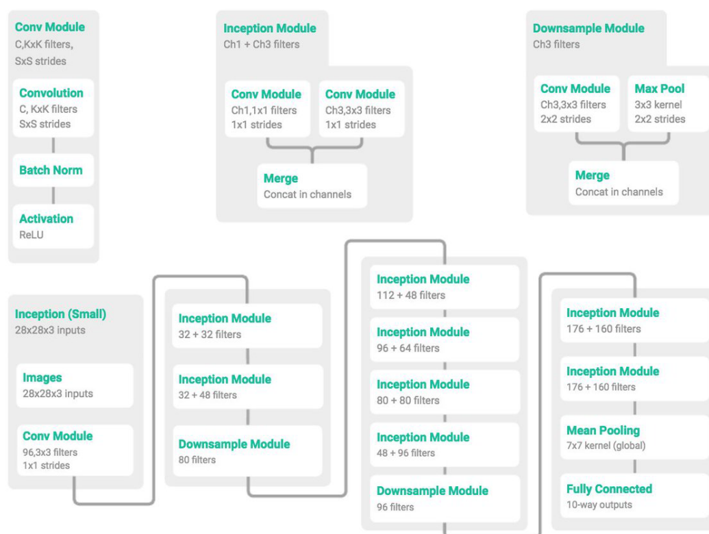
Figure 11.2: The Miniception architecture consists of building blocks including a convolution module, Inception module, and Downsample module. These modules are put together to form the overall architecture.
