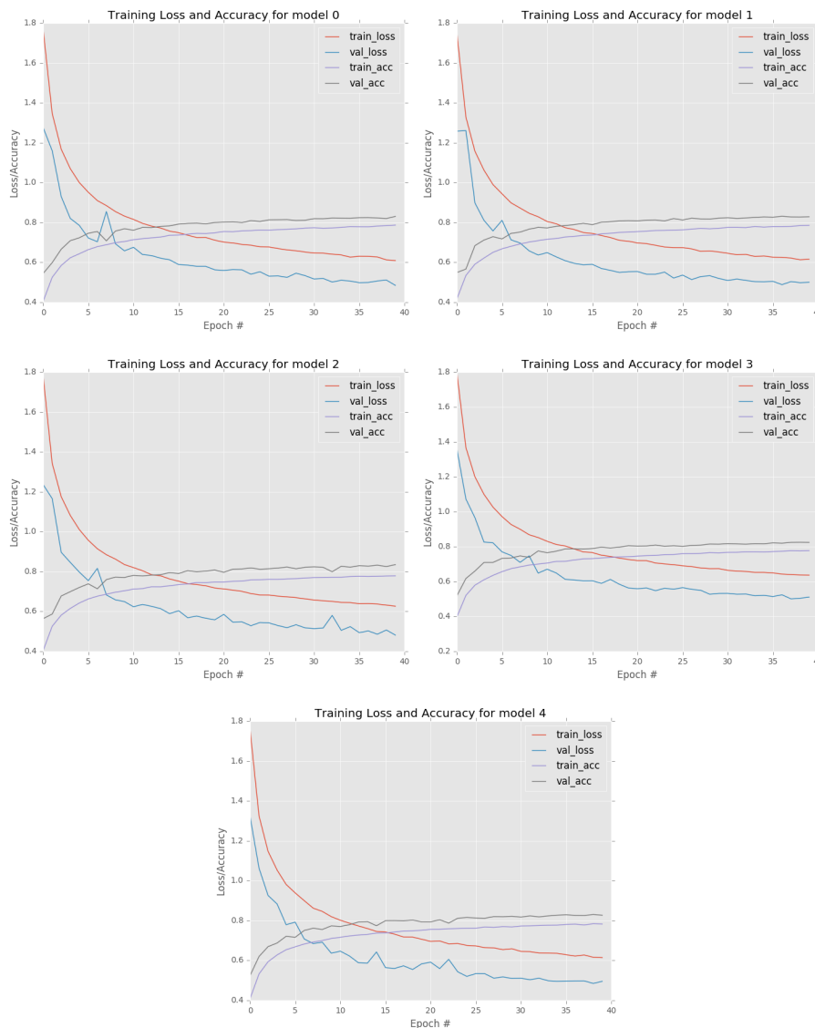
Figure 6.3: Training and validation plots for each of the five networks in our ensemble.
