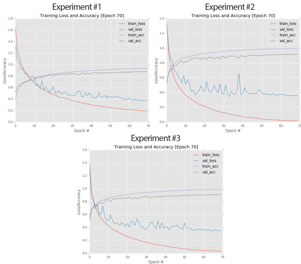
Figure 11.7: Top-left: Learning curves for Experiment #1. Top-right: Plots for Experiment #2. Bottom: Learning curves for Experiment #3. Our final experiment is a good balance between the first two, obtaining 90.81% accuracy, higher than all of our previous CIFAR-10 experiments.
