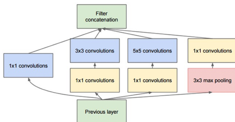
Figure 11.1: The original Inception module used in GoogLeNet. The Inception module acts as a “multi-level feature extractor” by computing 1 \times 1 , 3 \times 3 , and 5 \times 5 convolutions within the same module of the network. Figure from Szegedy et al., 2014 [17].
