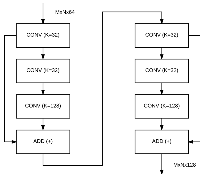
Figure 12.2: An example of two stacked residual modules where one feeds into next. Both modules learn K = 32, 32, and 128 filters, respectively. Notice how the dimensionality is reduced during the first two CONV layers then increased during the final CONV layer.
