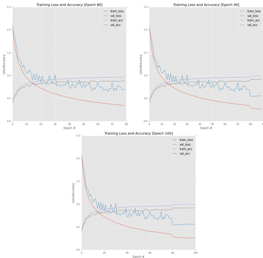
Figure 12.6: Top-left: First 80 epochs when training ResNet on CIFAR-10 in Experiment #3. Top-right: Next 10 epochs. Bottom: Final 10 epochs.
