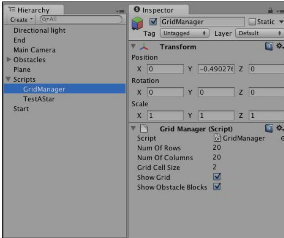
GridManager script
