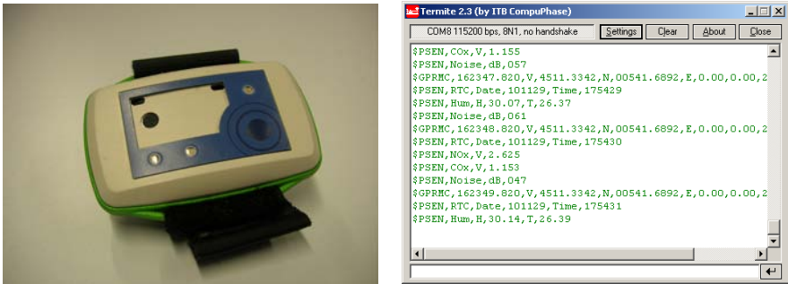
Fig. 3.5 City SensPod and an Impression on Raw Data Collection
