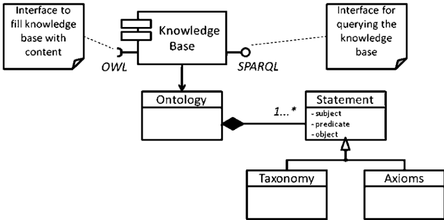
Fig. 12.8 The EURIDICE Knowledge Base Conceptual Model
