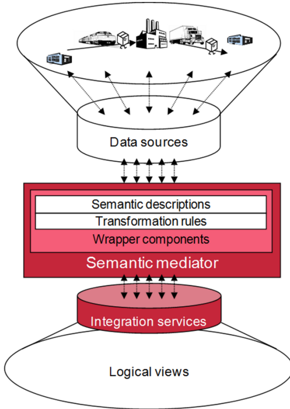
Fig. 6.3 Concept of a Service-oriented, Ontology-based Mediator
