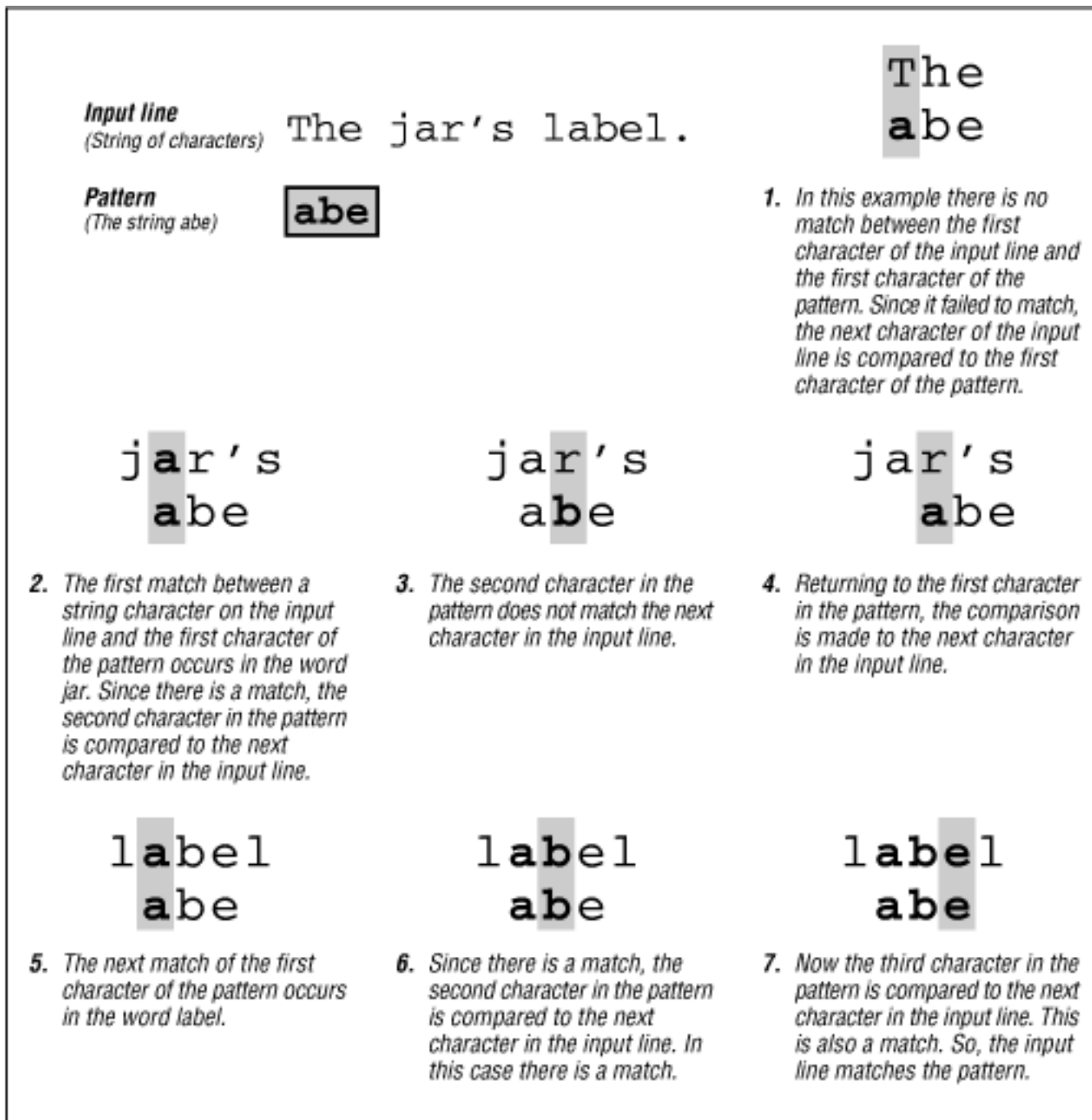
Figure 3.1: Interpreting a regular expression
