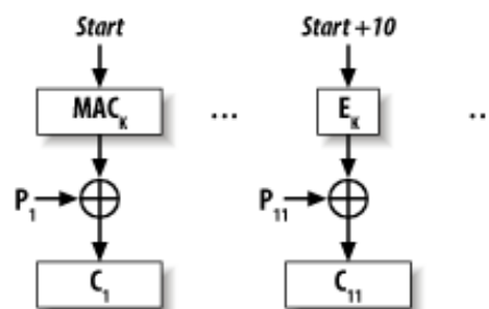
Figure 6-7. Encrypting with a MAC in counter mode
