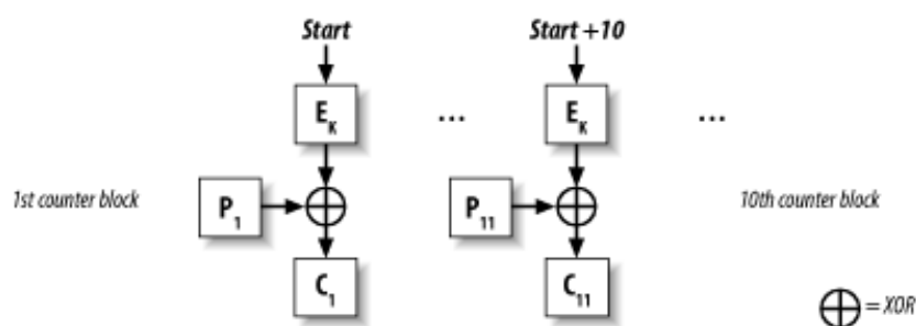
Figure 5-4. Counter (CTR) mode
