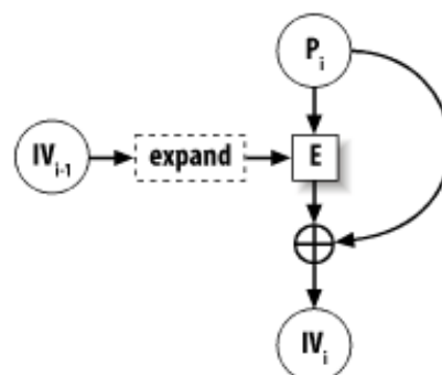
Figure 6-2. The Matyas-Meyer-Oseas construct
