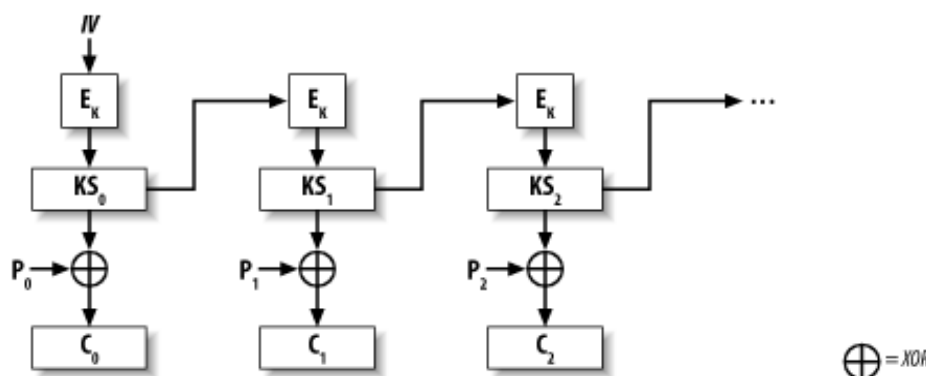
Figure 5-3. OFB mode
