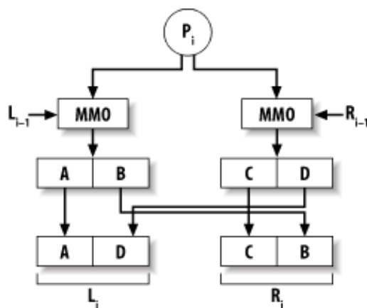
Figure 6-3. The MDC-2 construct
