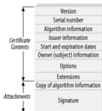
Figure 10-2. Contents of a certificate
