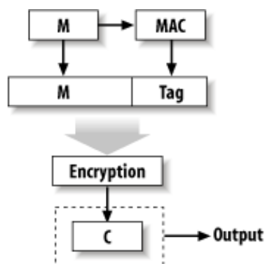
Figure 6-5. The authenticate-then-encrypt paradigm
