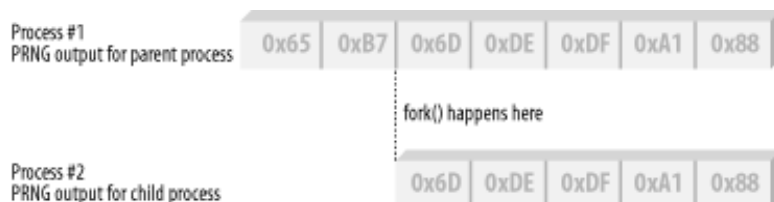
Figure 1-2. Consequences of not reseeding PRNGs after calling fork()
