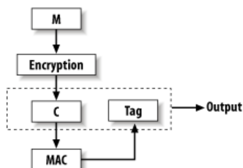
Figure 6-4. The encrypt-then-authenticate paradigm
