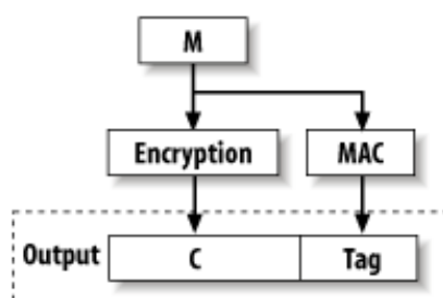
Figure 6-6. The authenticate-and-encrypt paradigm
