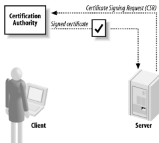
Figure 10-4. Obtaining a certificate from a CA
