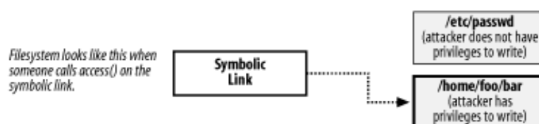
Figure 2-1. Stage 1 of a TOCTOU race condition: Time of Check
