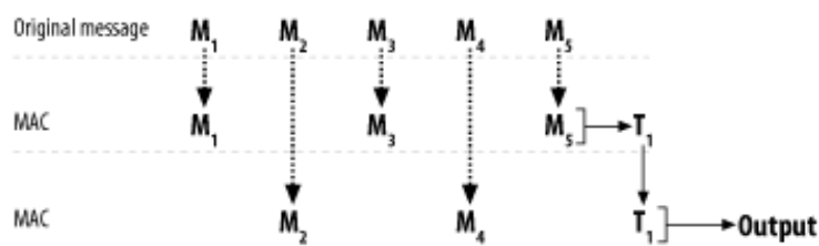
Figure 6-8. Properly interleaving MACs
