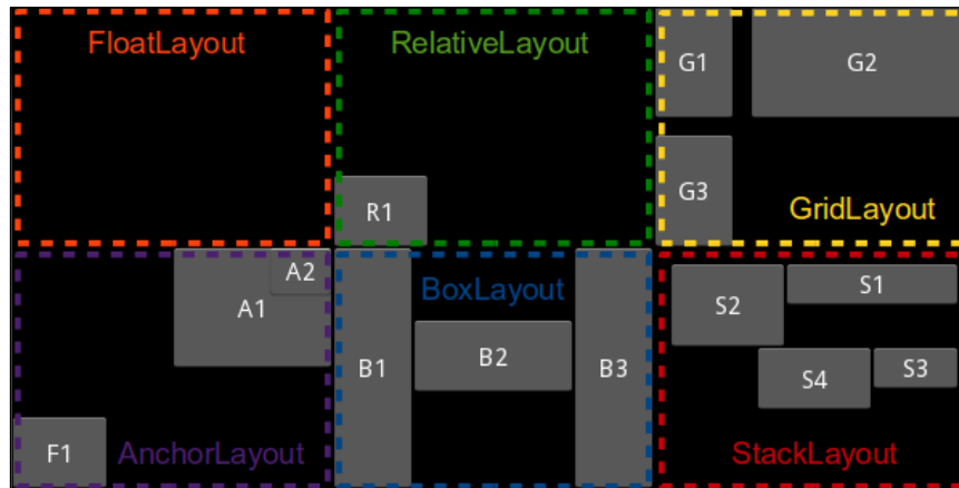
Embedding layouts
