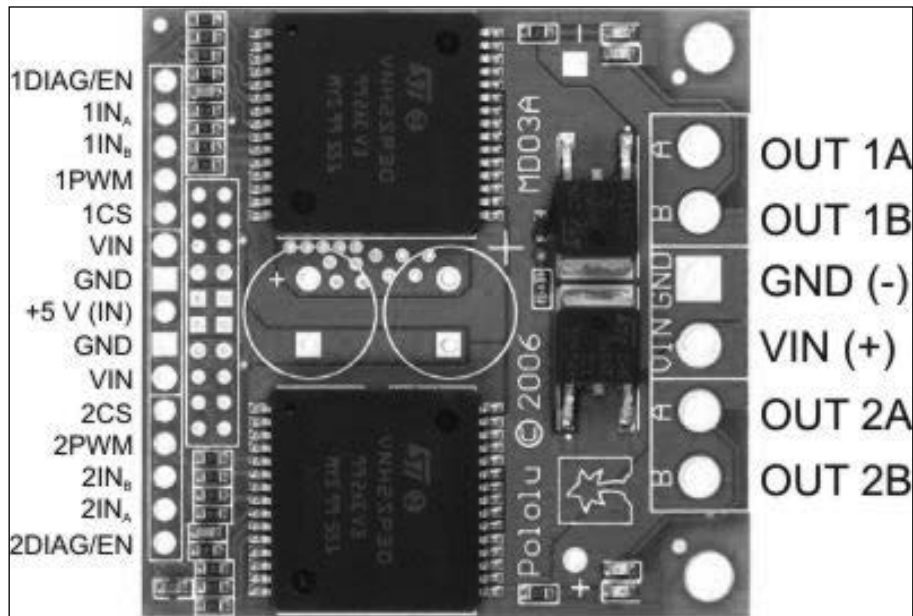
Dual VN12SP30 Motor Driver Carrier MD03A
