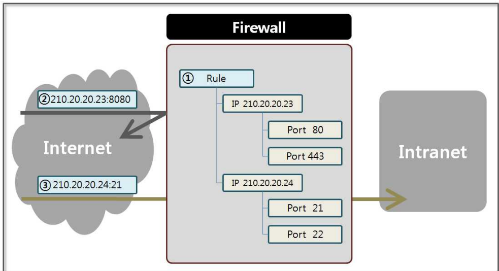
Figure 4-2 Firewall Concept Diagram
