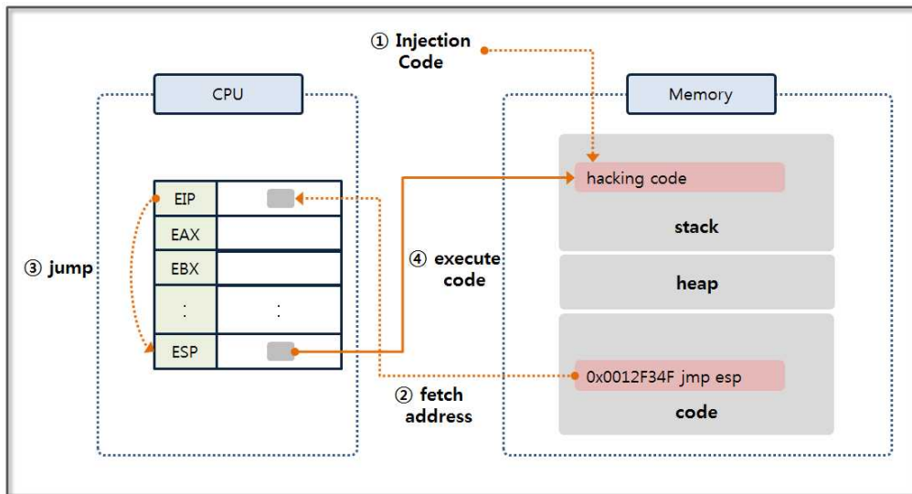
Figure 5-18 Stack Based Buffer Overflow behavior
