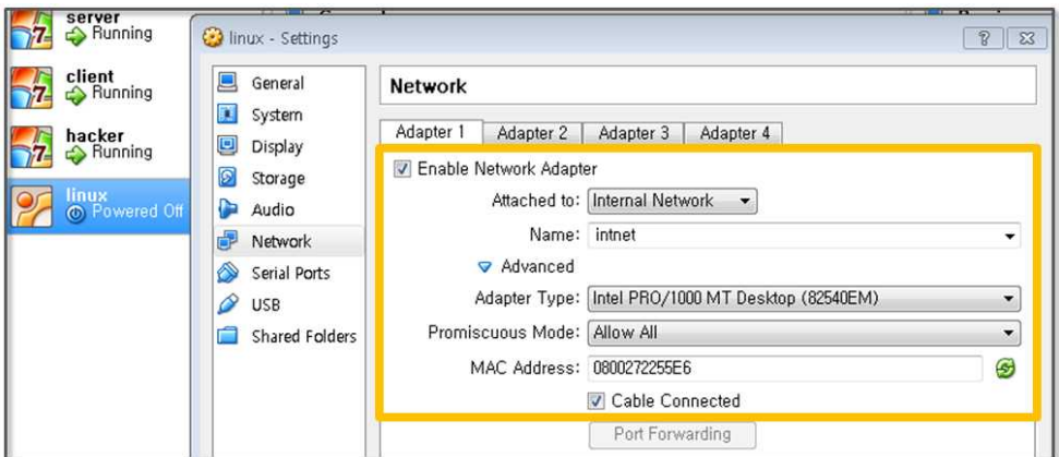
Figure 4-55 Virtual Box Network Setting
