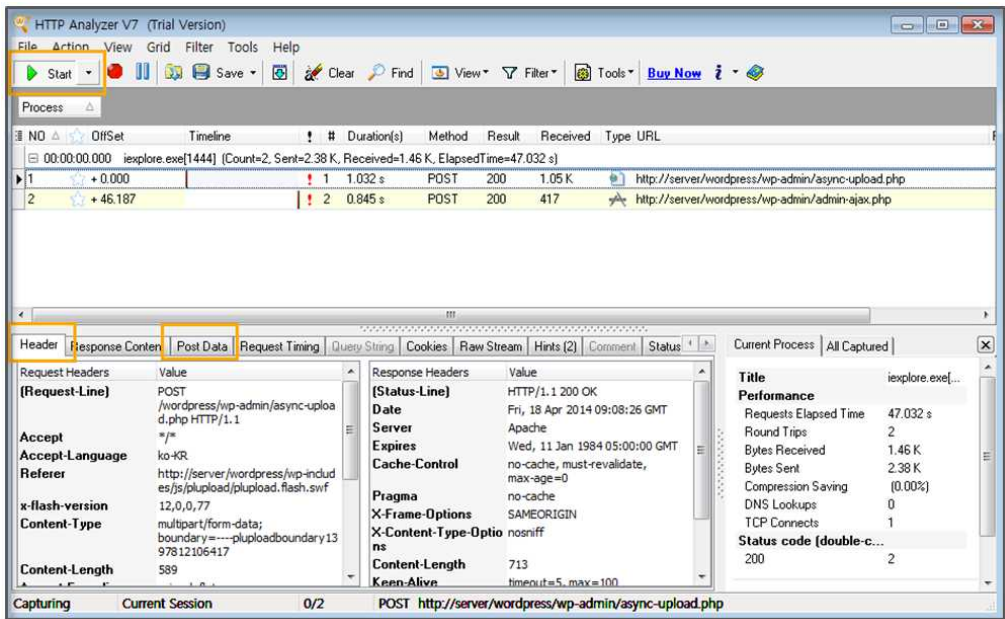
Figure 3-42 HTTP Analyzer Execution Screen
