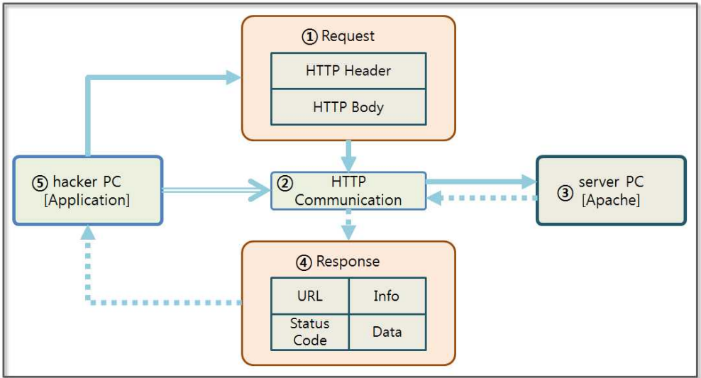
Figure 3-33 Python Web page Call Process
