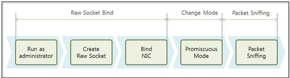
Figure 4-29 Packet Sniffing Procedure
