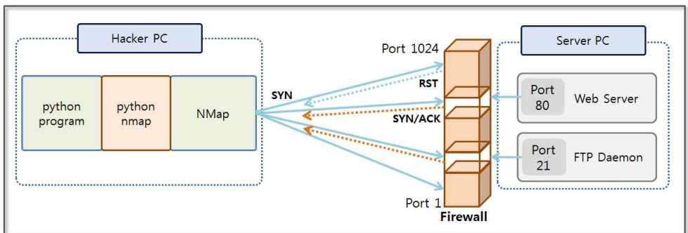
Figure 4-19 TCP SYNC SCAN of NMap
