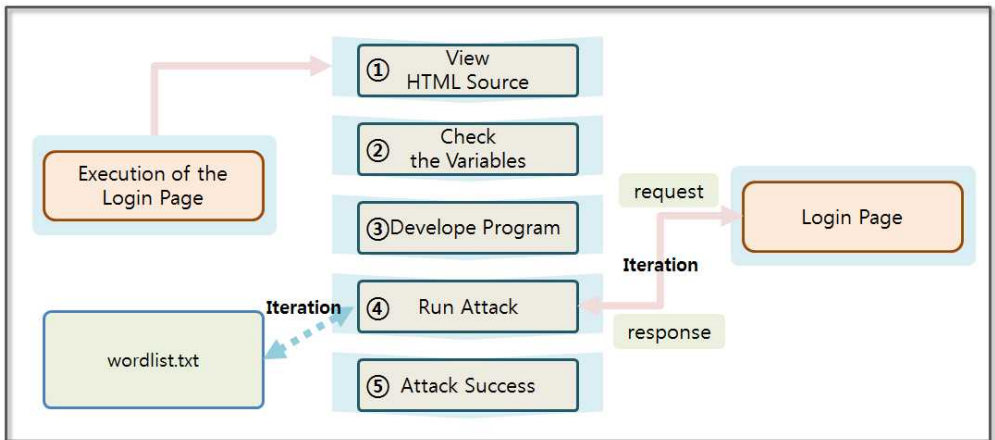
Figure 3-37 Password Cracking Concept
