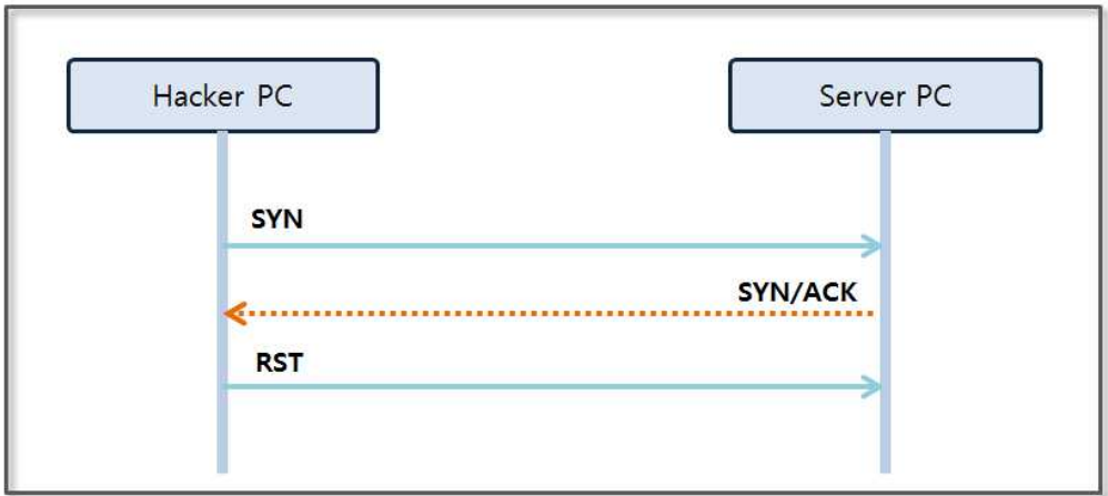
Figure 4-18 TCP SYN SCAN
