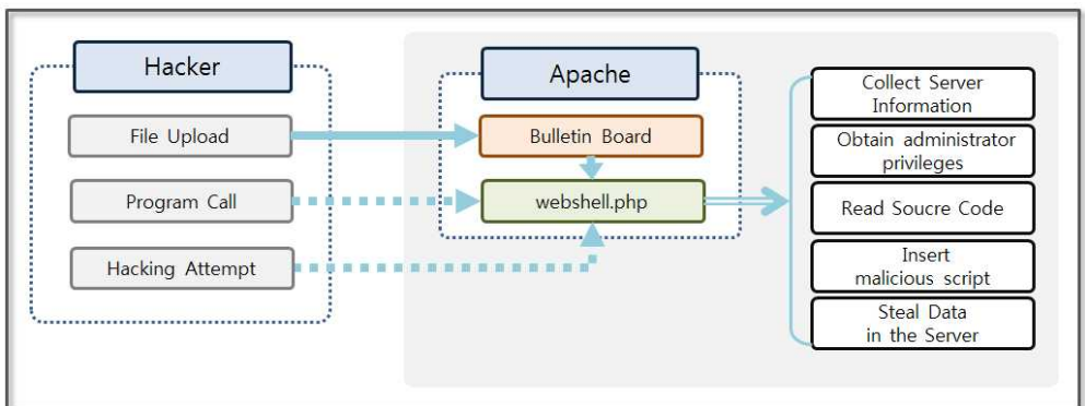
Figure 3-40 Web Shell Hacking Concept
