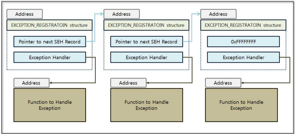
Figure 5-26 Behavior of the SEH chain
