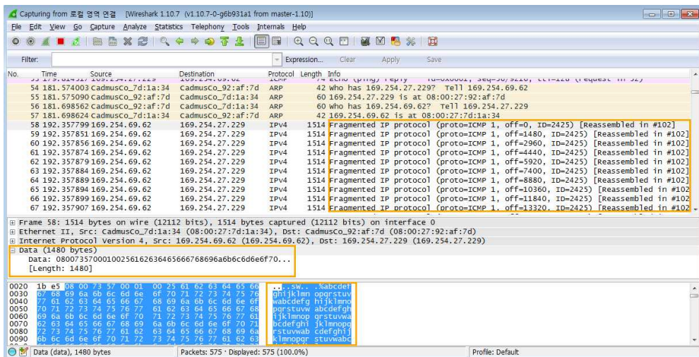
Figure 4-46 WireShark Packet Capture
