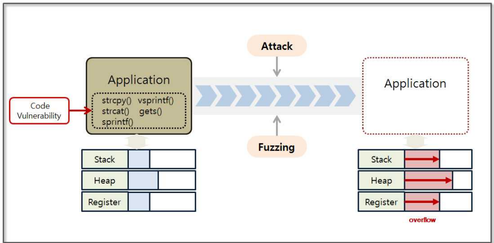
Figure 5-16 Basic Concept of a Buffer Overflow
