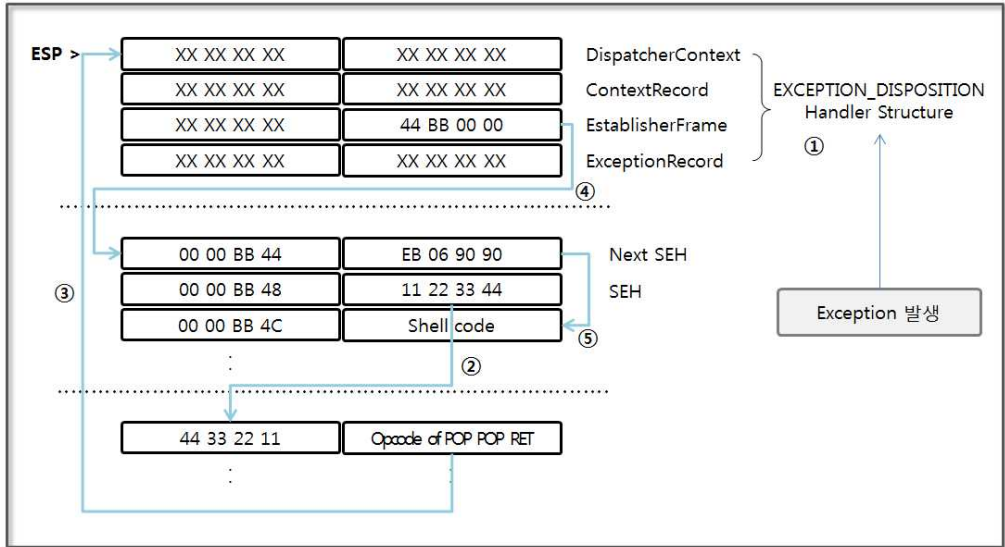
Figure 5-27 Behavior of the SEH Chain
