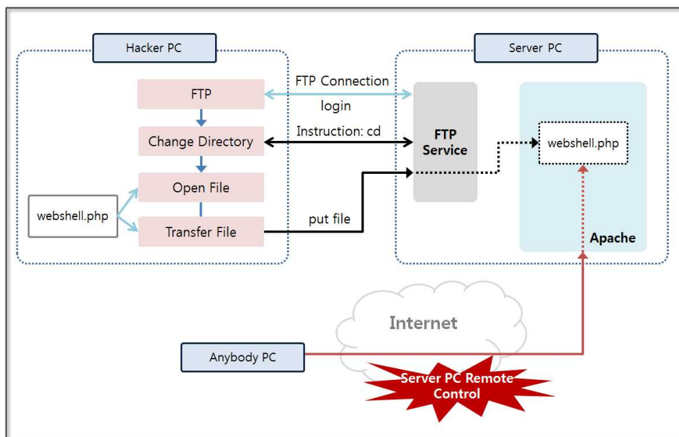
Figure 4-25 FTP Web Shell Attack
