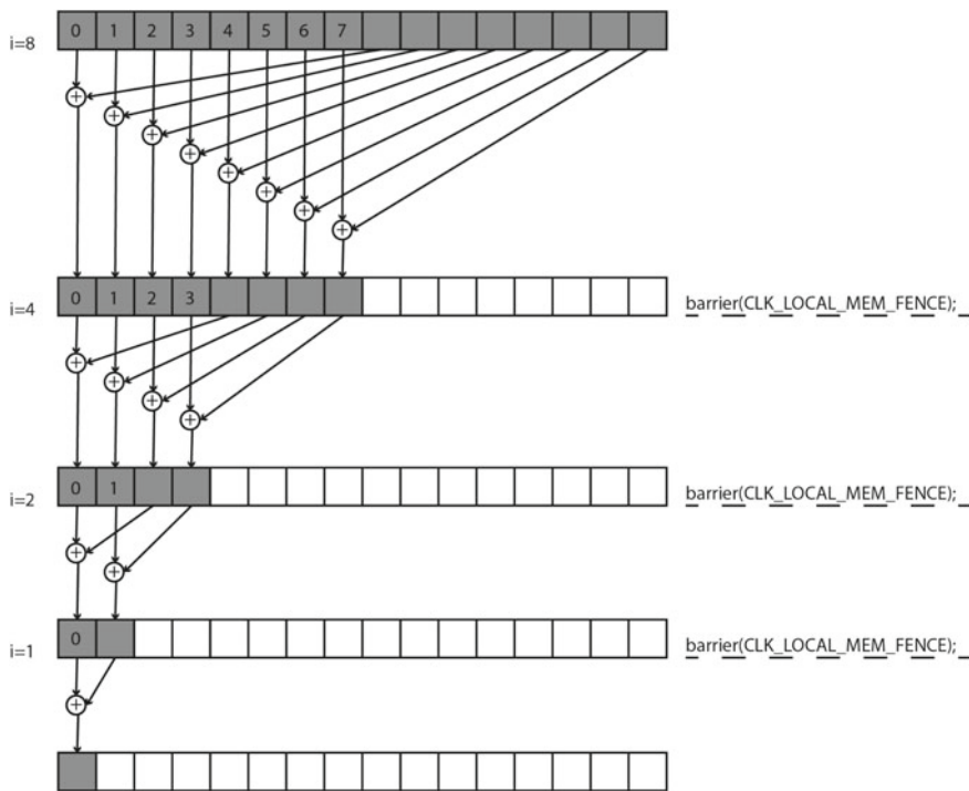
Fig. 5.12 Summation reduction
