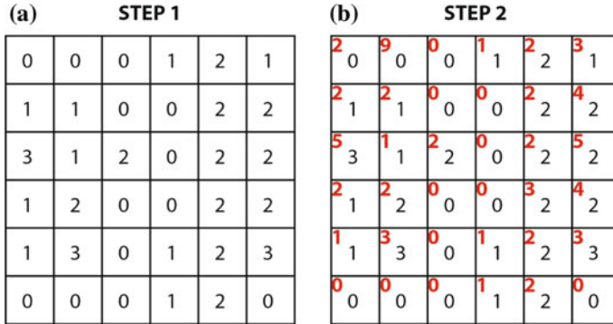
Fig. 8.4 a) Energies of the pixels. b) Cumulative energies
