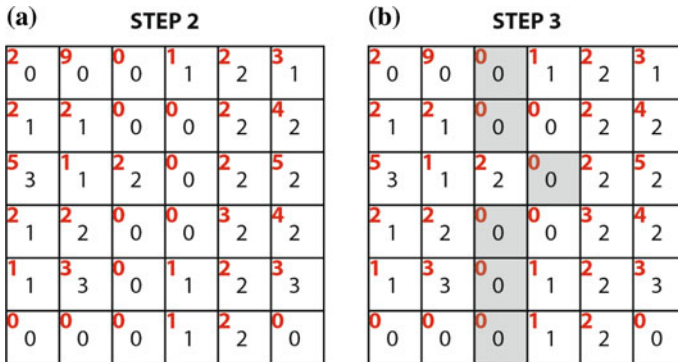
Fig. 8.6 a) Cumulative energies. b) The seam (in grey) with the minimal energy
