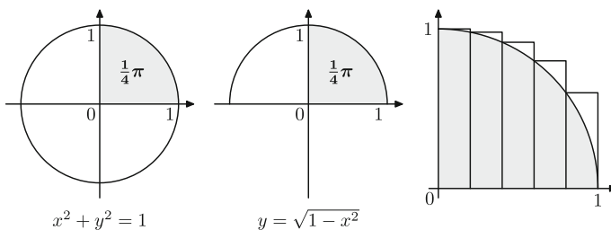
Fig. 3.12 Integrating y = \sqrt{1 - x^2} numerically from 0 to 1
