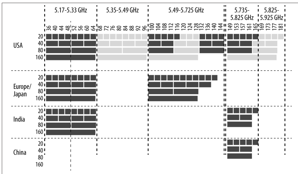
Figure 2-3. Available channel map for 802.11ac
