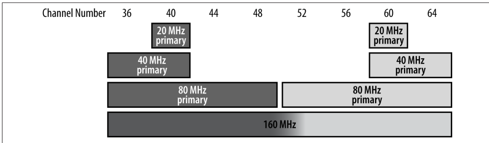
Figure 3-6. Coexistence of multiple networks in the same frequency space
