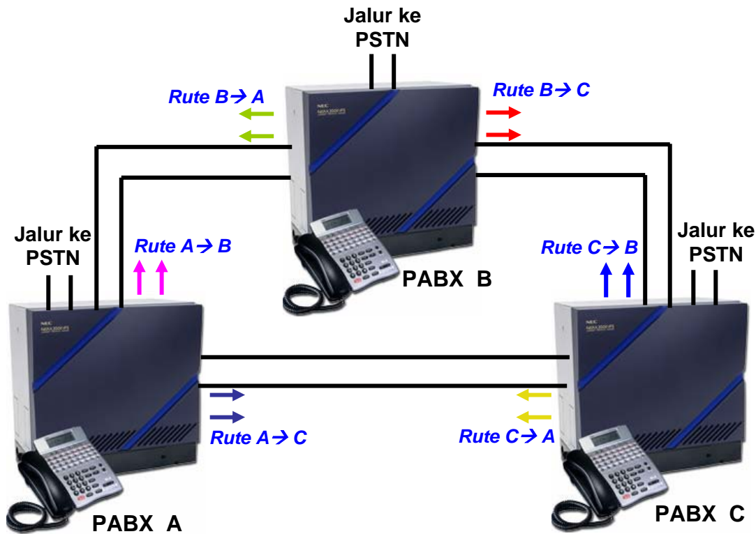
Gambar 9.1. Integrasi 3 PABX
