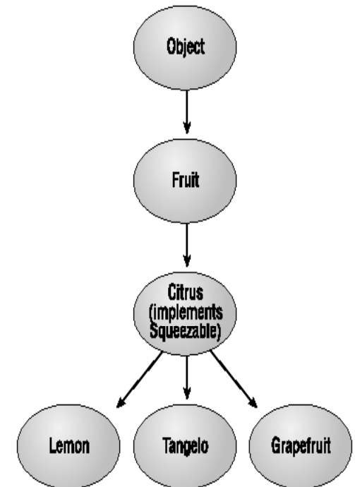
A simple class hierarchy
