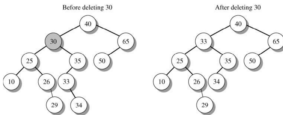
Replacing deleted value 30 with replacement value 33 and attaching right subtree 34.
